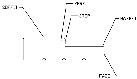
WOOD FRAME PROFILE DETAIL 2X SCALE
