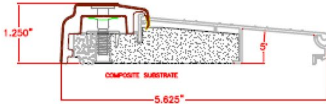
AFCO P-2000 ADJUSTABLE SILL (A-280 EXTRUSION)
