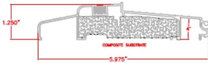
OUTSWING SILL
