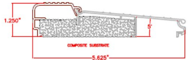
A-280 1 1/4" FIXED CAP SILL
